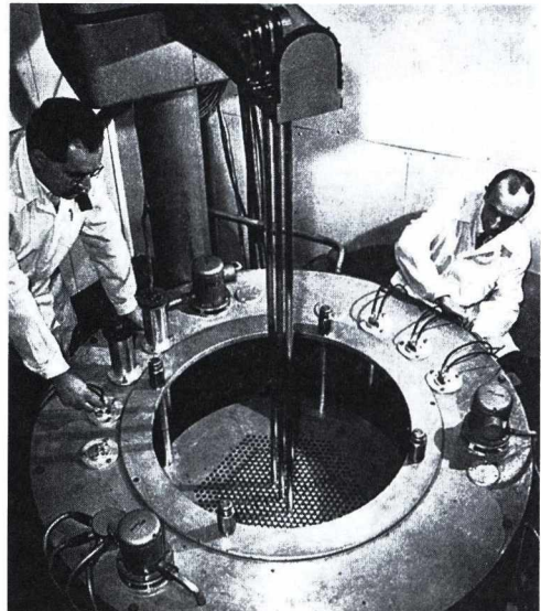
ZR-2
